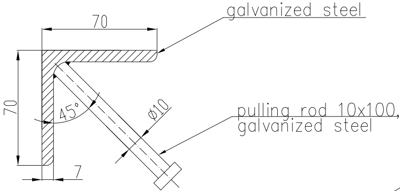
Angle 70x70x7 reinforced galvanized steel Section Scale 2:1
