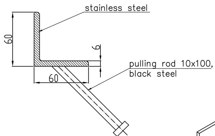
Angle 60x60x6 reinforced stainless steel Section Scale 2:1
