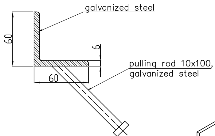
Angle 60x60x6 reinforced galvanized steel Section Scale 2:1
