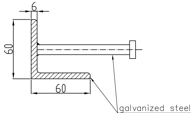
Angle 60x60x6 reinforced galvanized steel Section Scale 2:1
