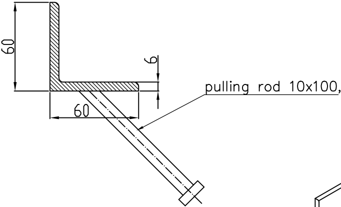
Angle 60x60x6 reinforced black steel Section Scale 2:1
