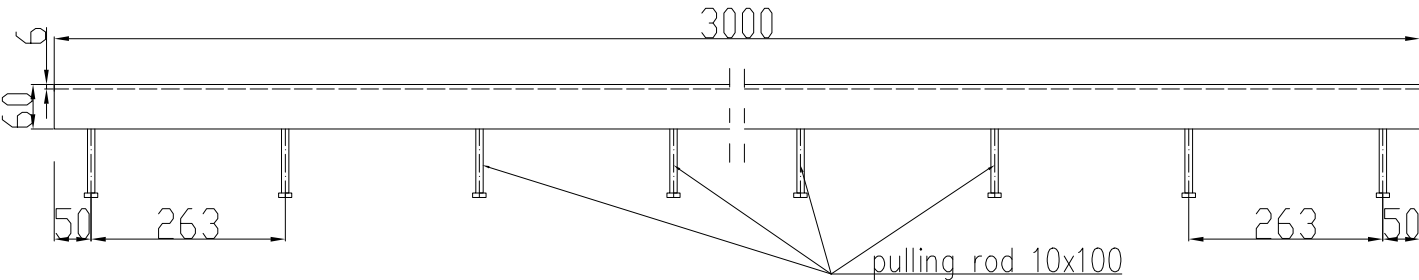
Angle 60x60x6 reinforced black steel L=3000
