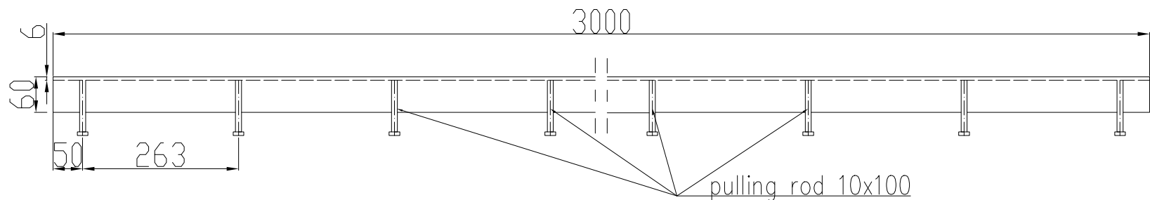
Top view Scale 1:2
