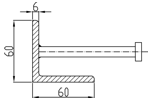
Angle 60x60x6 reinforced black steel Section Scale 2:1
