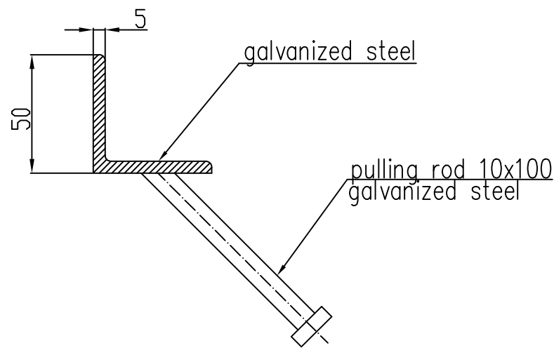
Angle 50x50x5 reinforced galvanized steel Section Scale 2:1
