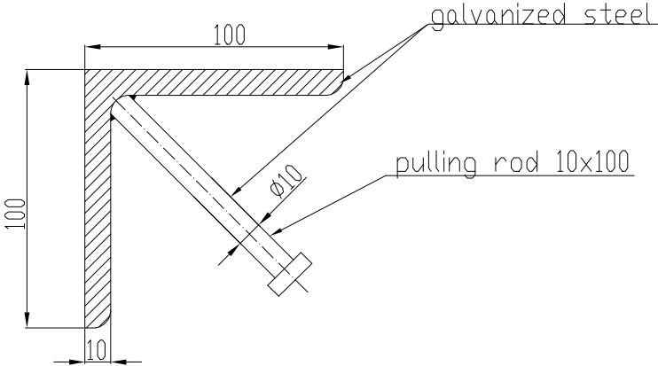
Angle 100x100x10 reinforced galvanized steel Section Scale 2:1
