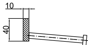
CONECTO Single Strip Joint 10NA40 Section
