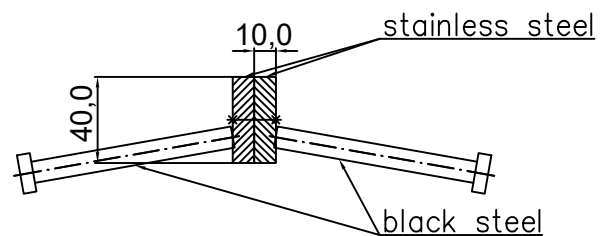
DOUBLE STRIP JOINT 10NA40 reinforced SECTION
