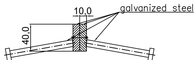
DOUBLE STRIP JOINT 10NA40 reinforced SECTION
