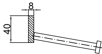
Conecto Single Strip Joint 08NA40 Section
