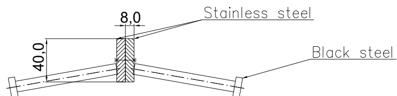
DOUBLE STRIP JOINT 08NA40 reinforced Section
