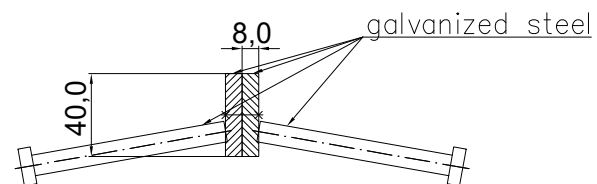
DOUBLE STRIP JOINT 08NA40 reinforced Section
