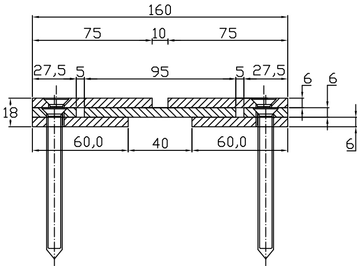
CONECTO SINUS 06NC160/18-R S40K10 Section
