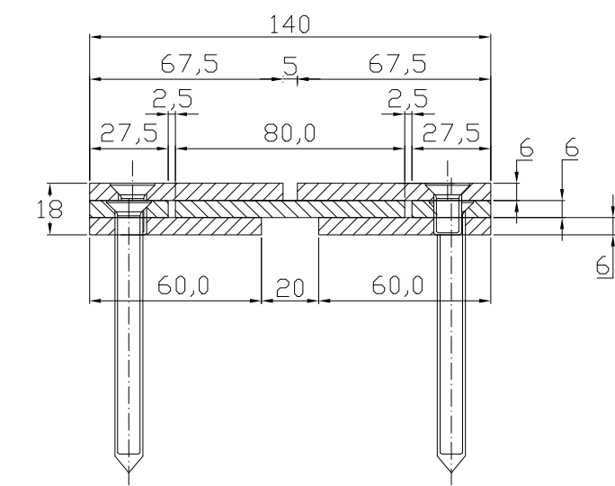
Conecto Sinus 06NC140/18-R S20K5 Section
