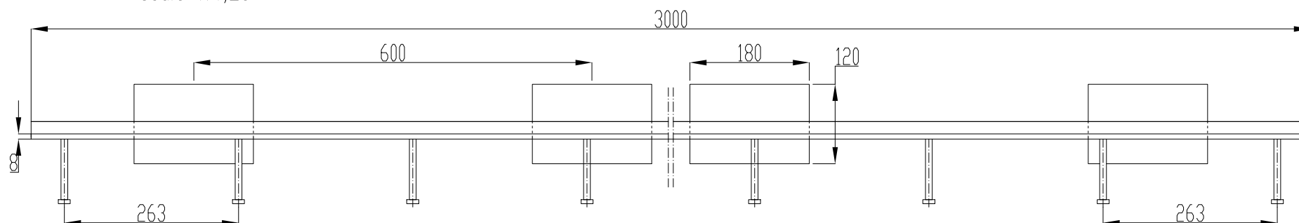
Conecto Omega 03NB-5D-T8 h=155/170 Top view scale 1:1,25
