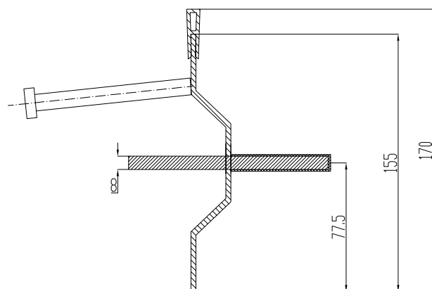
Conecto Omega 03NB-5D-T8 h=155/170 Section scale 2:1
