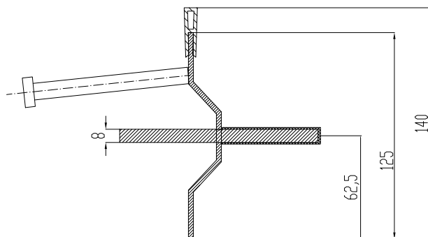
Conecto Omega 03NB-5D-T8 h=125/140 Section scale 2:1
