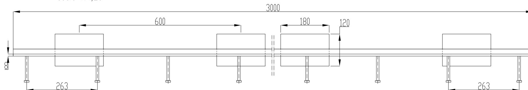
Conecto Omega 03NB-5D-T8 h=125/140 Top view scale 1:1,25
