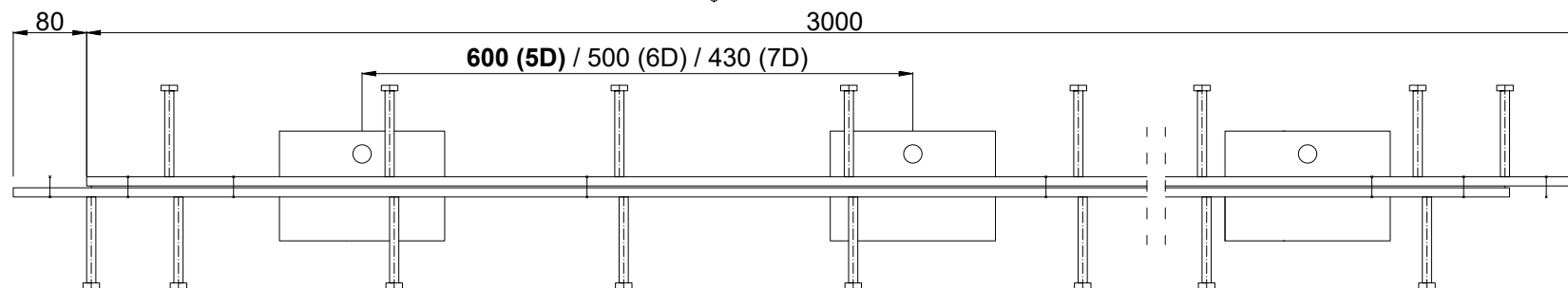
Conecto Dowel 10NA40-5D-T8 h=225 PC L=3000, galvanized steel version
