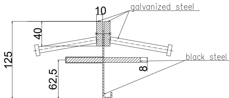
Conecto Dowel 10NA40-5D-T8 h=125 galvanized steel version SECTION SCALE 2:1
