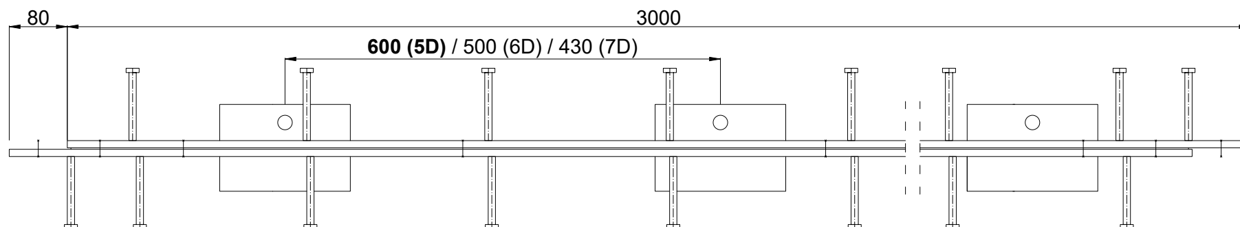
Conecto Dowel 10NA40-5D-T8 h=125 PC L=3000, galvanized steel version
