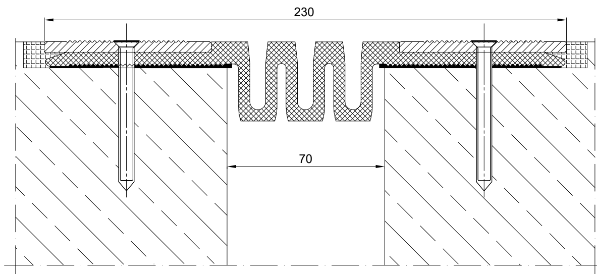
CONECTO PARK SL 230.70.W SECTION
