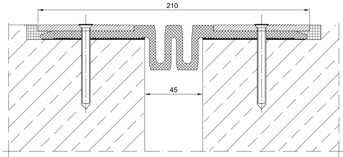
CONECTO PARK SL 210.50.W SECTION
