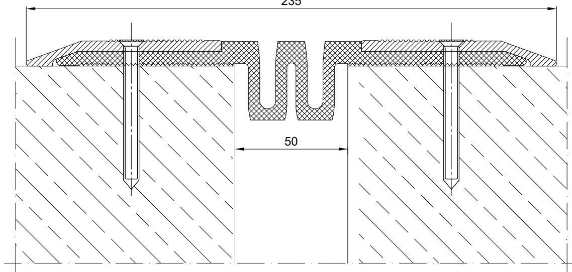
CONECTO SL 210.50.N SECTION
