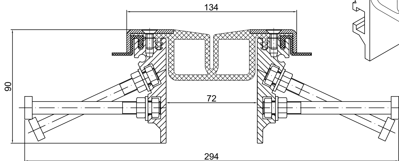
CONECTO GA 88.45.90& S SECTION
