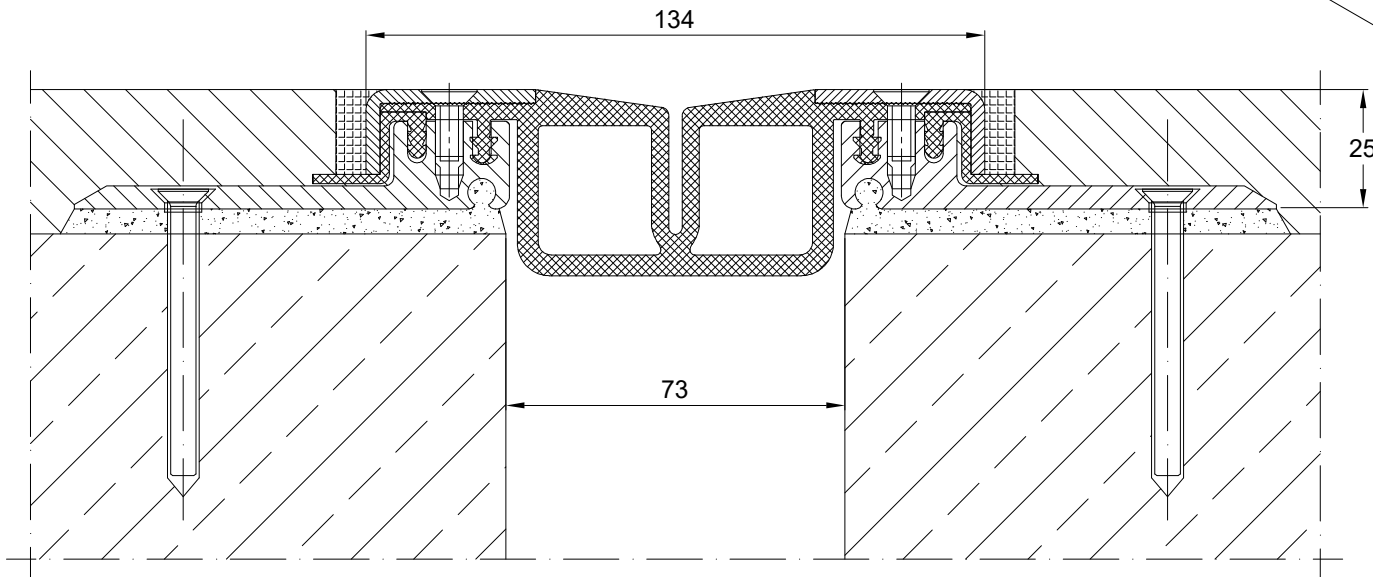
CONECTO GA 88.45.25 S SECTION
