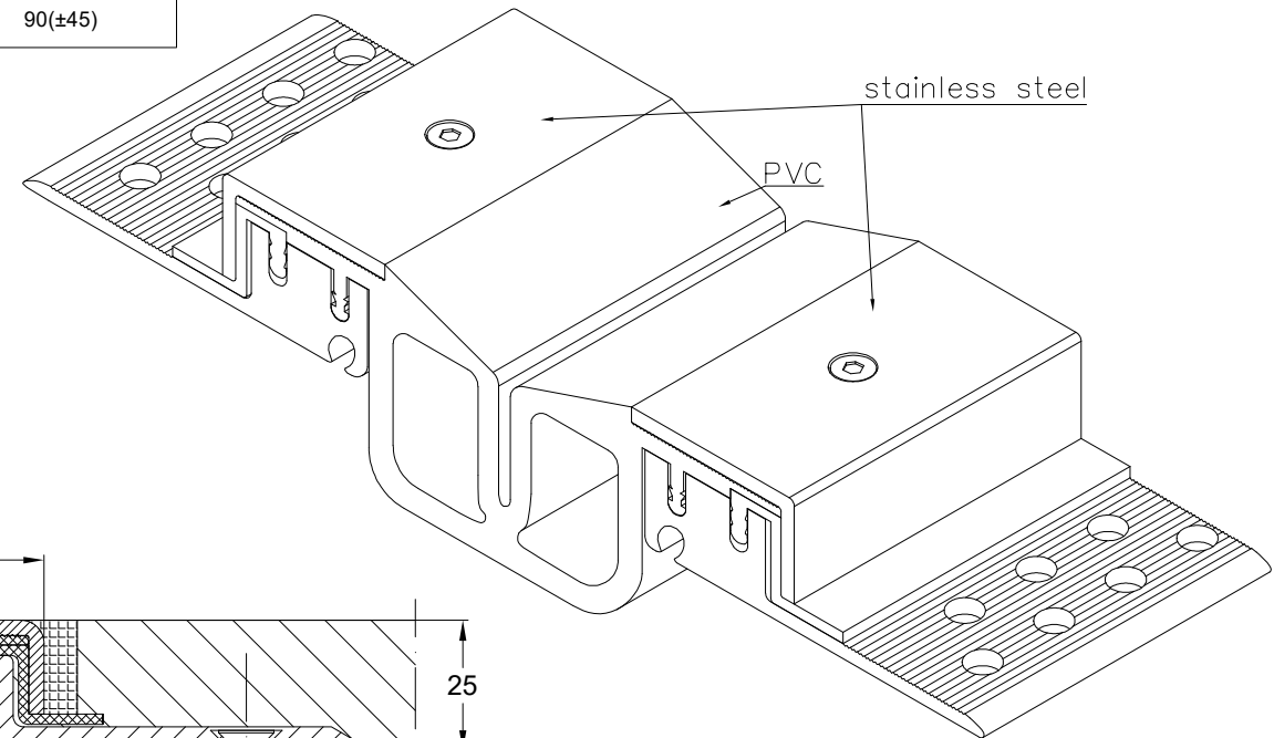
CONECTO GA 88.45.25 S VIEW
