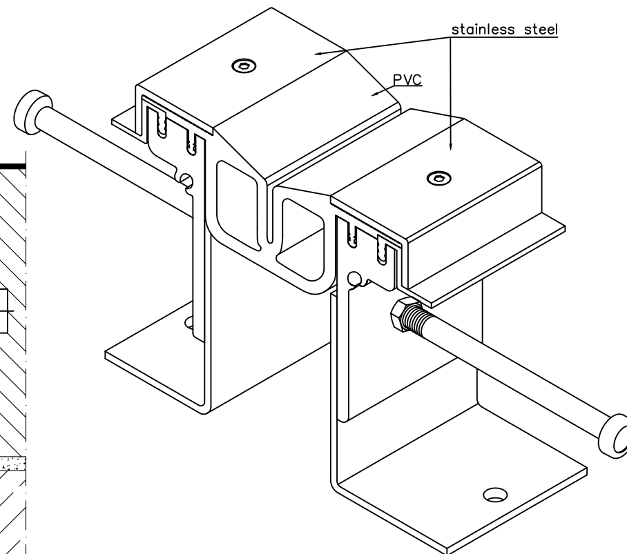
CONECTO GA 88.45.120& S with galvanized studs VIEW
