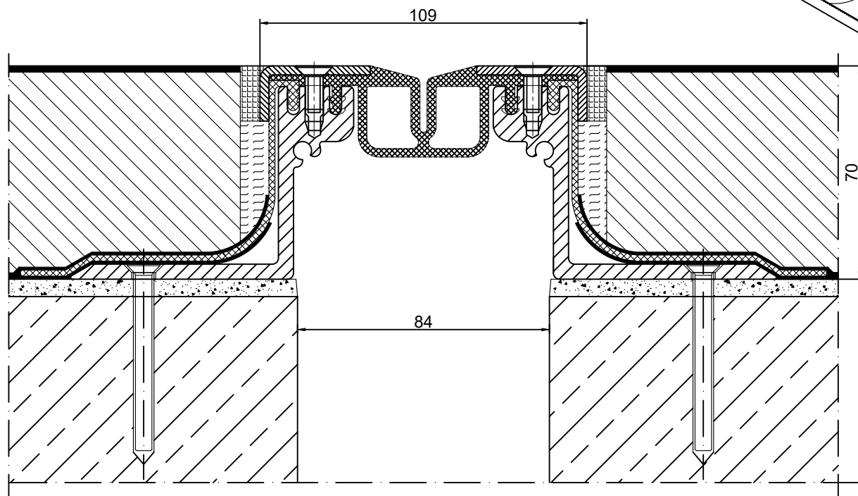
CONECTO GA 63.30.70L SECTION
