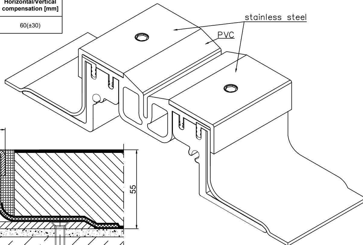
CONECTO GA 63.30.55 L VIEW
