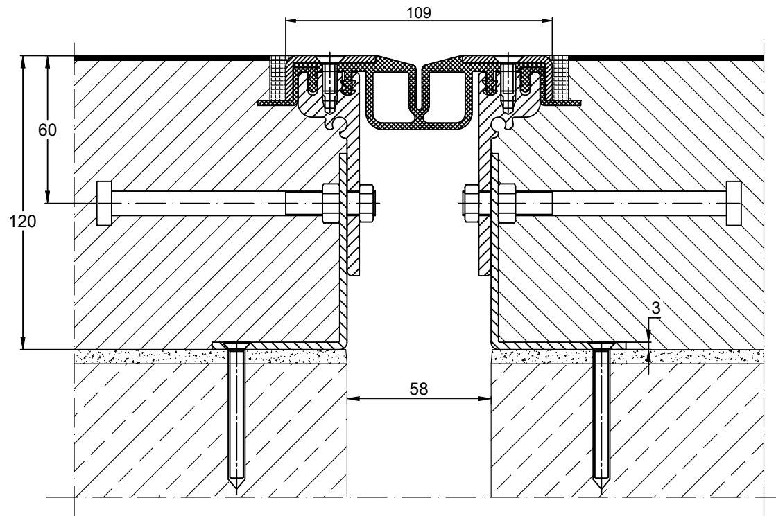
CONECTO GA 63.30.120& S with galvanized studs SECTION
