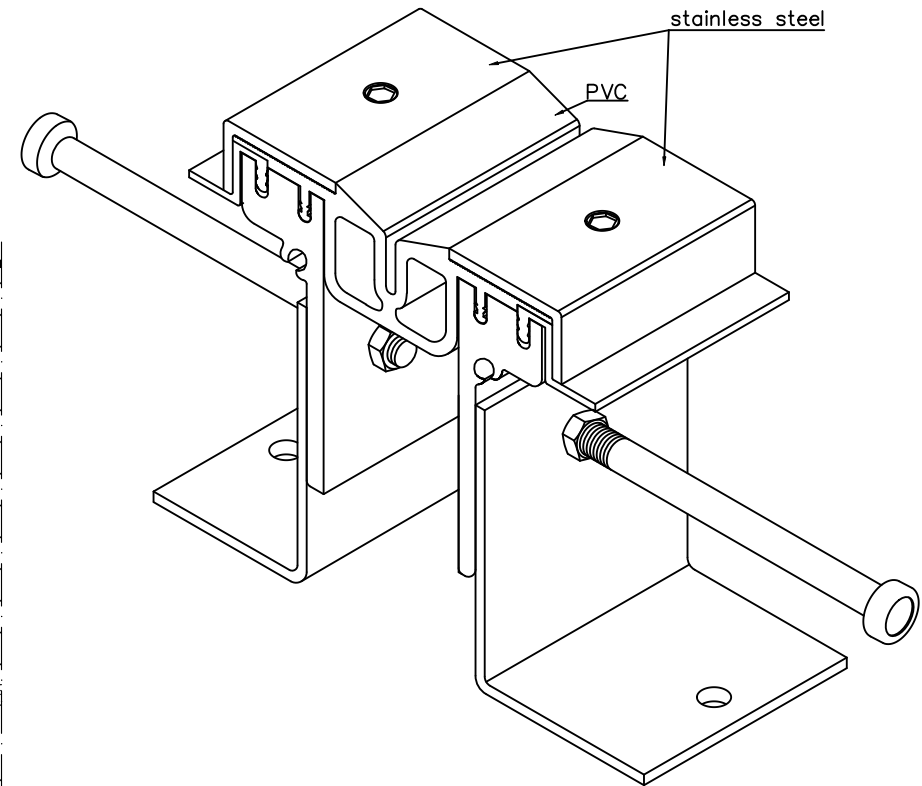
CONECTO GA 63.30.120& S with galvanized studs VIEW
