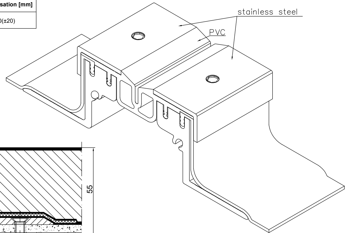
CONECTO GA 50.20.55 L VIEW
