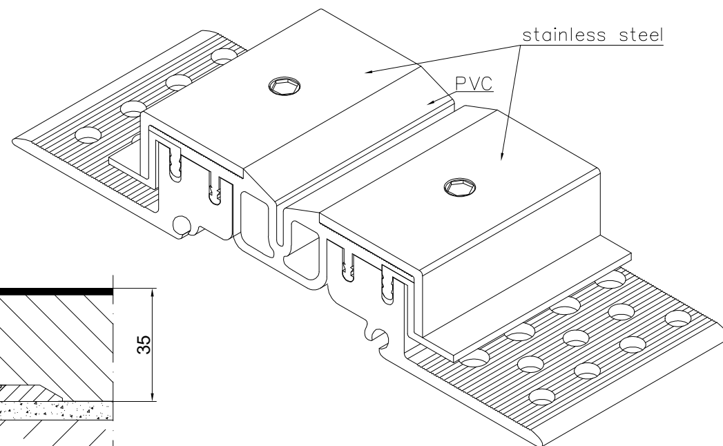
CONECTO GA 50.20.35 S VIEW
