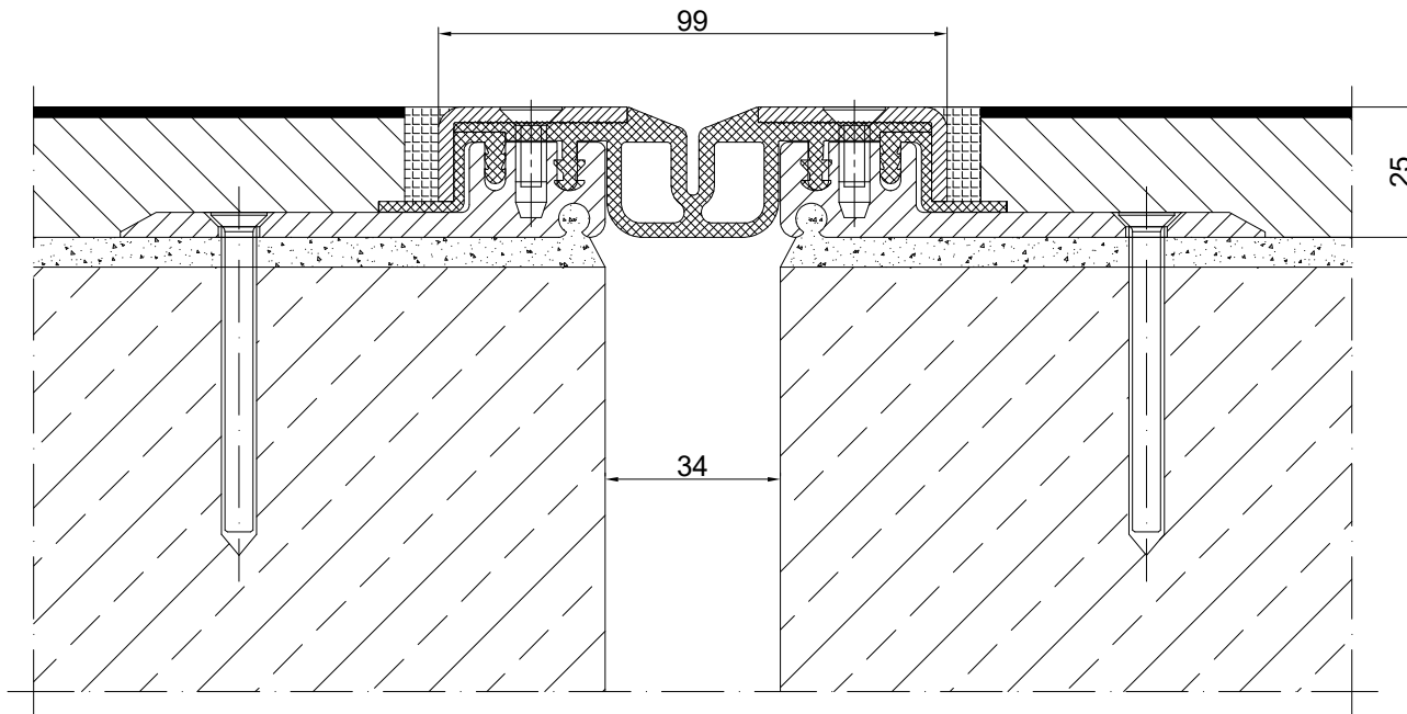
CONECTO GA 50.20.25 S SECTION
