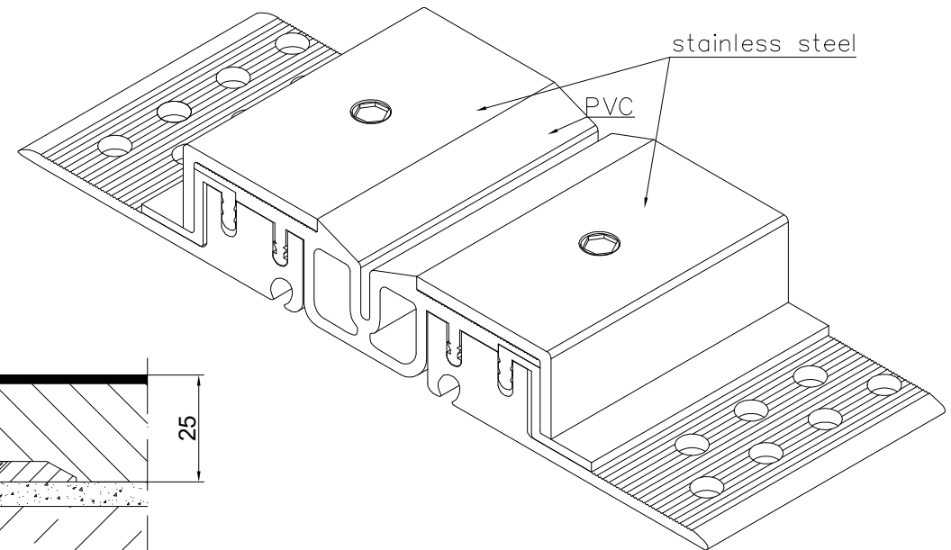
CONECTO GA 50.20.25 S VIEW
