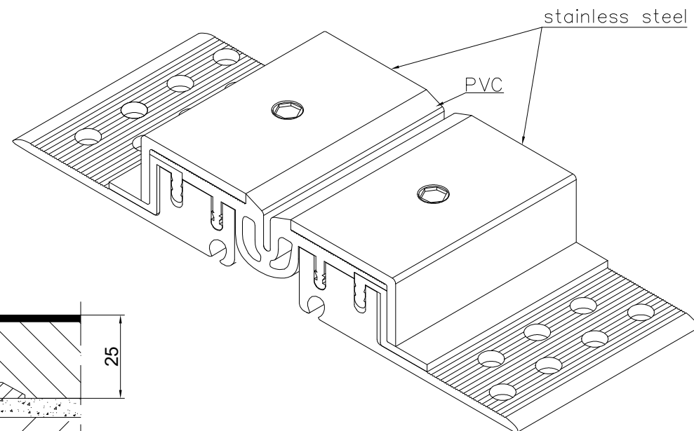
CONECTO GA 43.10.25 S VIEW
