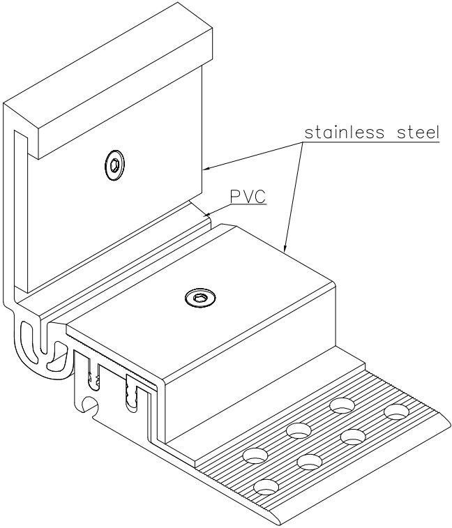
CONECTO GA 43.10.25S CV PERSPECTIVE VIEW
