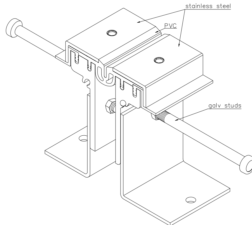
CONECTO GA 43.10.120& S with galvanized studs VIEW
