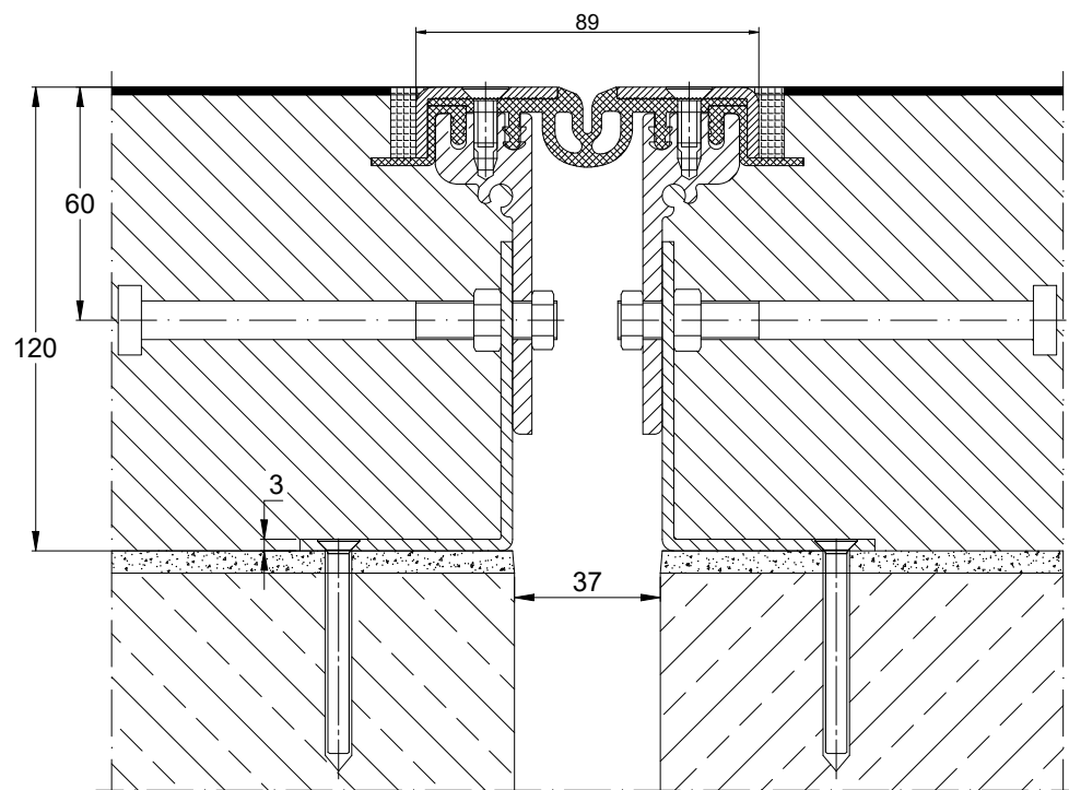
CONECTO GA 43.10.120& S with galvanized studs SECTION
