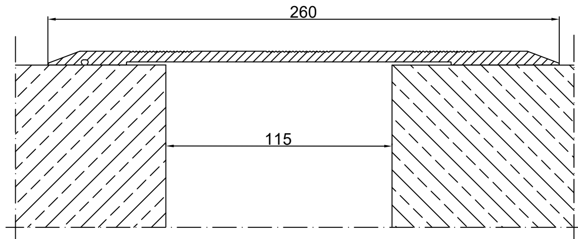
CONECTO CS 260 VIEW SCALE 1: 4
