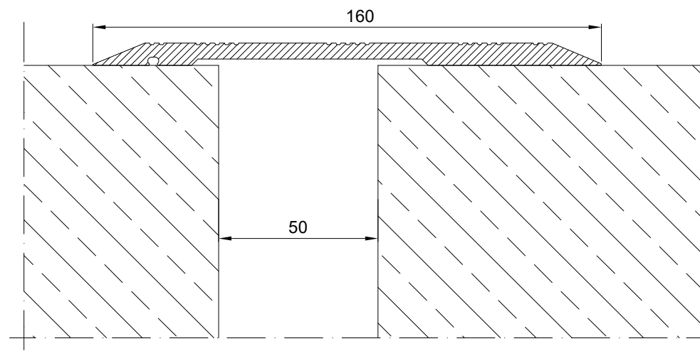
CONECTO CS 160 VIEW SCALE 1:4
