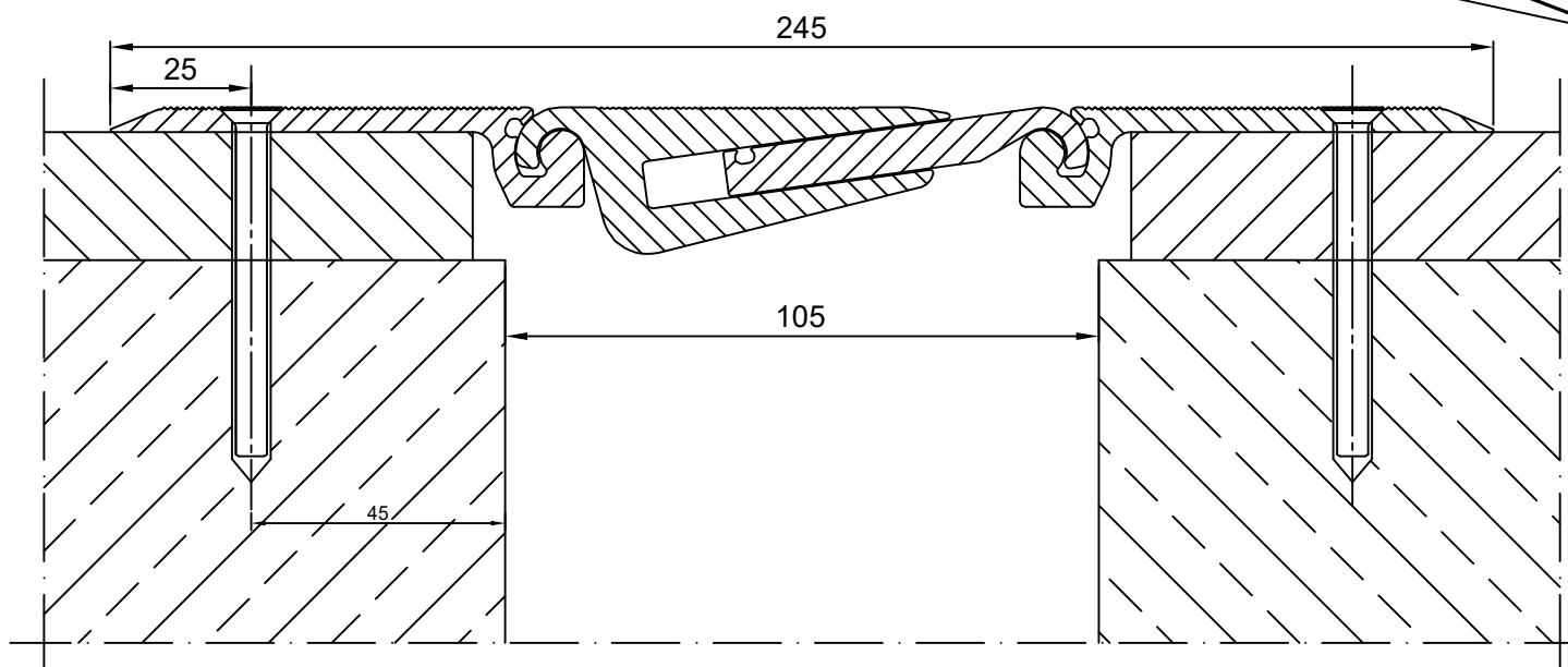
Expansion joint Conecto AL 110.15.N
